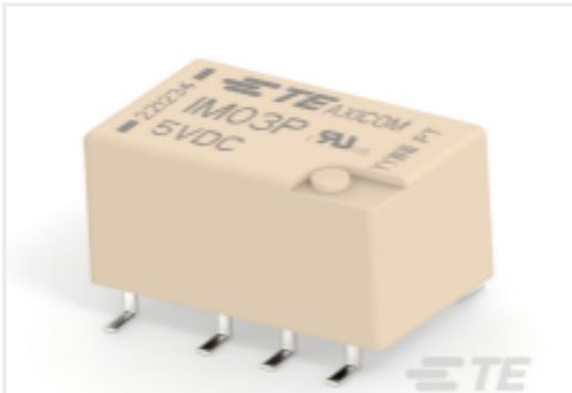
TE 产品编号5-1462039-5 IM03PGR=IM RELAY 140mW 5V
