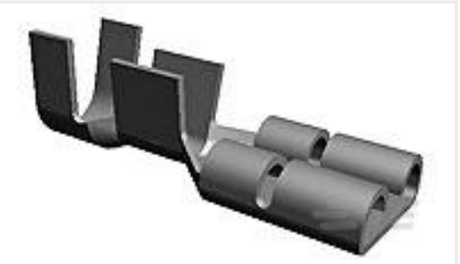
TE 产品编号444334-2 250 FASTON REC 22-18 AWG TPBR
