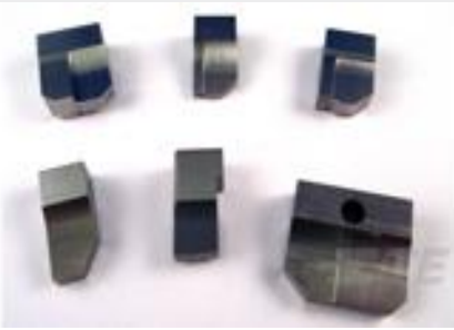
TE 产品编号2-1333229-2 ANVIL, COMBINATION SPECIAL
