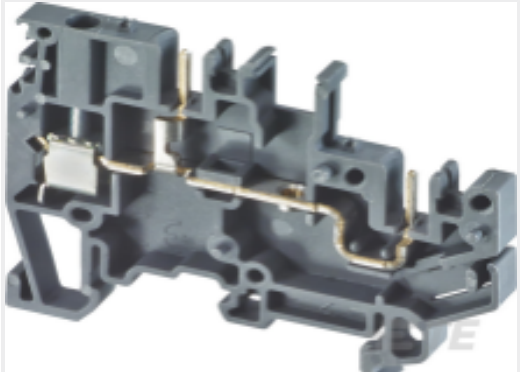
TE 产品编号1SNA400817R0000 MA2.5/5-2CPE
