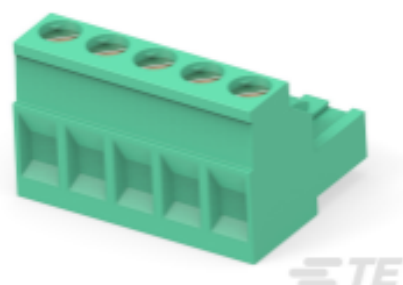
TE 产品编号 796634-5 5 POS 5.08MM R/A PLUG, TRM BLK
