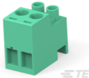
TE 产品编号 1986880-2 2P MODULAR, 2 WAY, SIDE STCK, 3.5 MM
