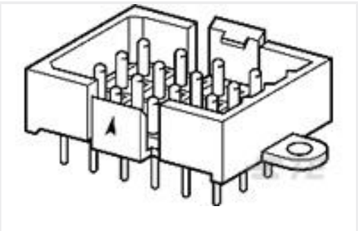
TE 产品编号1986569-1 METRIMATE PIN HDR ASY,12P LF
