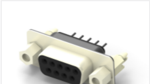
TE 产品编号2301838-2 AMPL REC HD20, VERT, 9P, B/L,4-40 S /LOCK
