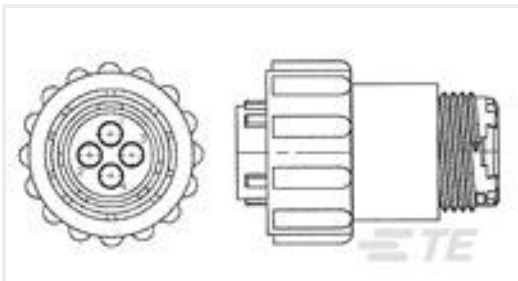
TE 产品编号1977878-1 SLD CPC PLUG ASY,11-4,STD SEX, UV RESIST
