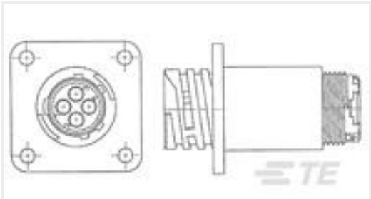
TE 产品编号788154-2 SLD CPC RCPT ASSY,11-4,REV SEX
