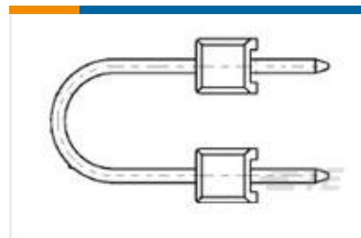
TE 产品编号2-1740617-4 AMP MODU II SOLDER STRAP
