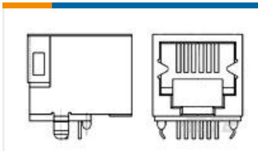
TE 产品编号1734723-1 RJ11,6P6C,SINGLE,DIP,W/O LED 6u"
