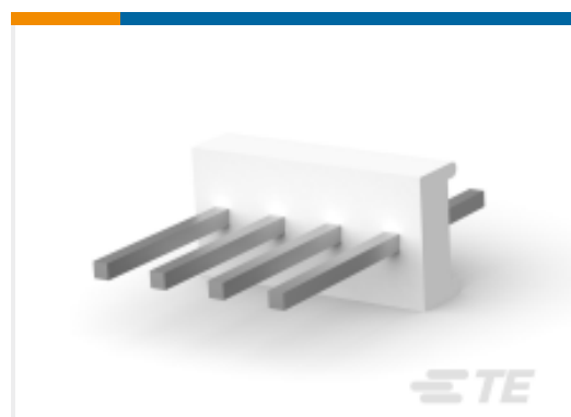
TE 产品编号3-647609-4 PCB Header: Polyester, Vertical, Unshrouded, No Mating Alignment
