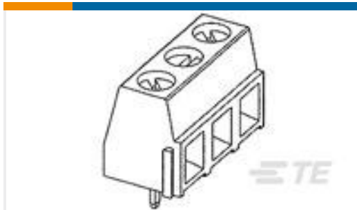
TE 产品编号282837-2 TERMI-BLOK PCB MOUNT 2P
