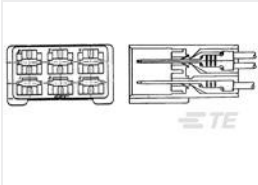
TE 产品编号171433-1 FF 250 TAB HSG 6P NYLON NAT
