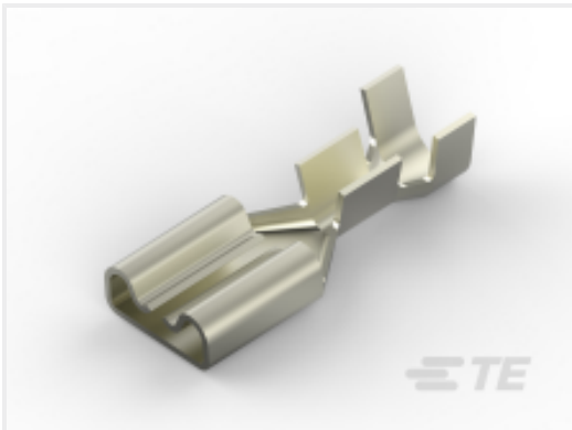
TE 产品编号2238196-3 FASTON 250 STD REC STR 18-14TPBR
