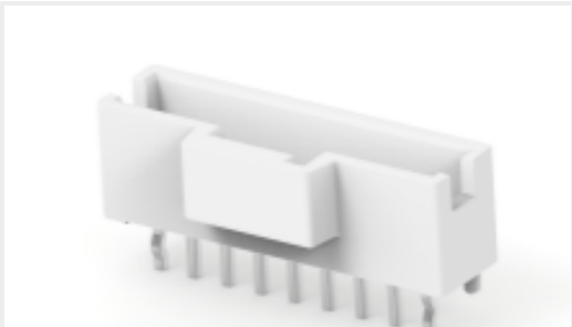
TE 产品编号1-2232826-9 SGI2.0 header assembly TH 9P,key A, NTL
