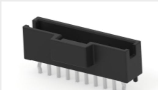
TE 产品编号5-2232826-0 SGI2.0 header assembly TH 10P,key B, BLK
