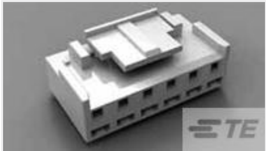
TE 产品编号3-1123722-9 3.96 EP PLUG HSG 9P(BLUE)
