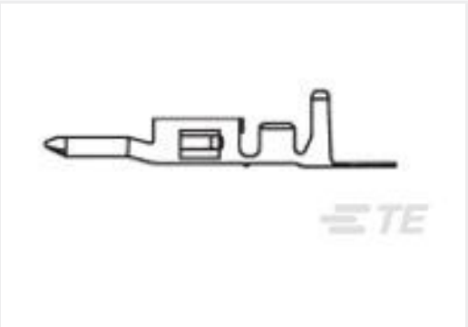
TE 产品编号2238016-1 VAL-U-LOK PIN BR SN 18-22AWG
