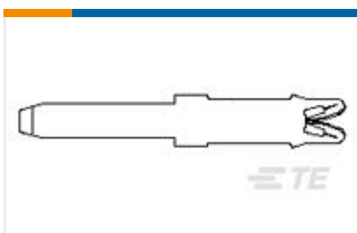
TE 产品编号1601194-2 .110X.032 TAB STD SIAMEZE
