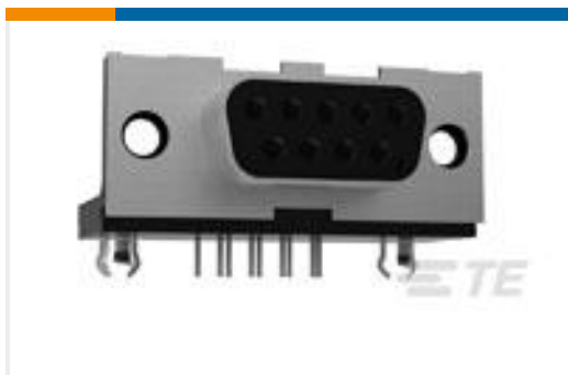
TE 产品编号3-106505-2 9P.HDP20 REC.ASSY.
