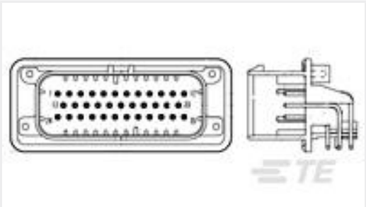
TE 产品编号1-776163-6 35POS,PIN DIA 1.3,HDR ASSY,90DEG, COD 6
