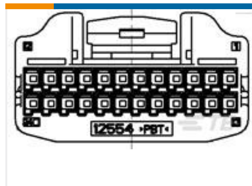
TE 产品编号1717118-1 0.64 III 32POS PLUG ASSY
