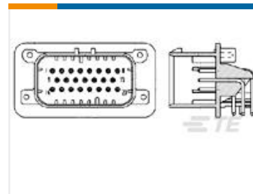
TE 产品编号776087-1 23POS,PIN DIA 1.3,HDR ASSY,90DEG, COD 1
