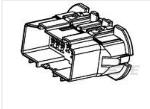
TE 产品编号1-936366-1 090/JPT 25P CAP ASSY(DTB-RS)
