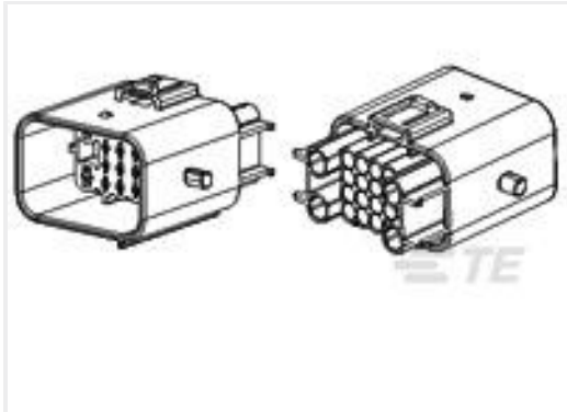
TE 产品编号936780-2 MT-II/JPT SLD 20P CAP HSG
