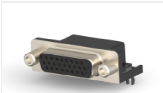
TE 产品编号2311768-1 AMPL REC, HD22, R/A, 26P, THREADED
