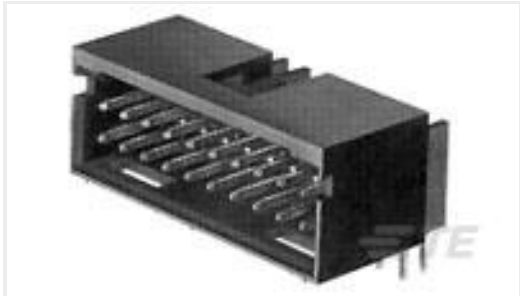
TE 产品编号5-103167-2 10 MODII HDR DRRA SHRD LF
