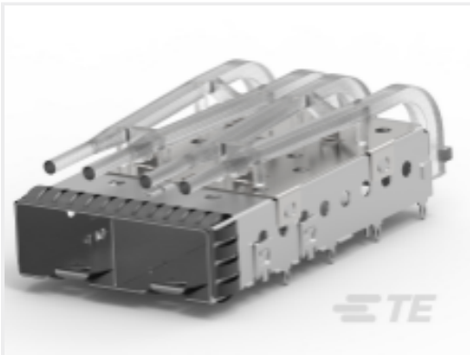
TE 产品编号 2007262-1 SFP+ 1x2 Cage Assembly, Light
