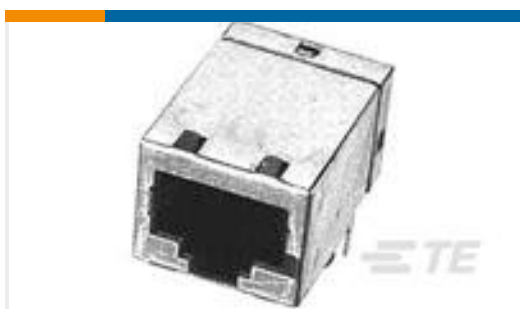
TE 产品编号1-1734264-3 M/J,RJ45,Side,8P8C,R/A,50u" Au, D3.2
