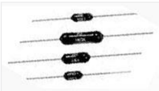
TE 产品编号1-1879621-6 H4P 43R 1% 50PPM
