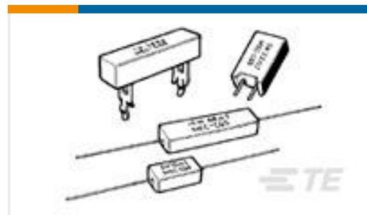
TE 产品编号1-1623789-3 SQM7 39R 5% (WIRE)
