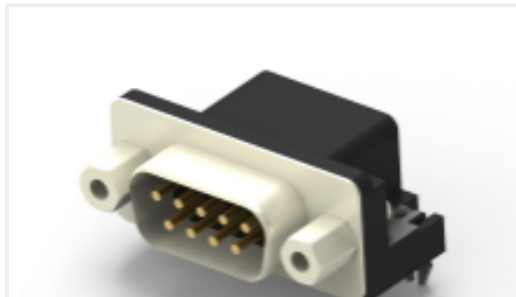
TE 产品编号2301843-2 AMPL PLUG HD20, R/A, 9P, B/L,4-40 S /LOCK
