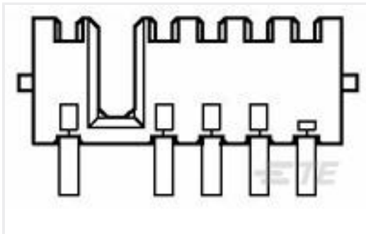
TE 产品编号1747367-1 RECEPTACLE ASSEMBLY 2.5MM PITCH BATTERY
