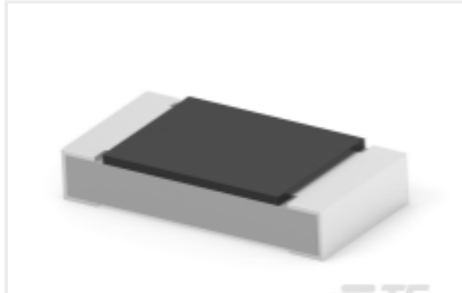
TE 产品编号3-2176583-7 RLC73PW 2B R133 1% 1K RL
