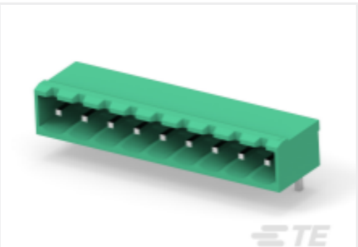
TE 产品编号2350513-9 9POS TB HDR 90 DEG, PITCH 5.0 & TL 4.5mm
