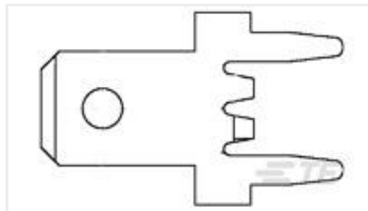
TE 产品编号1217332-1 187 FASTON,PCB TAB,TCBR
