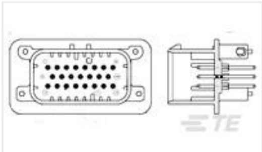
TE 产品编号776228-2 23POS,PIN DIA 1.3,HDR ASSY, 180DEG,COD 2
