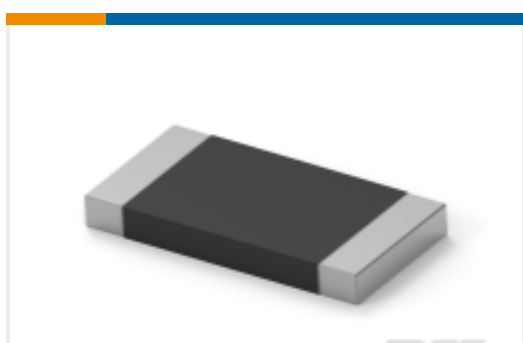
TE 产品编号7-2176422-9 TLRP 2512 3.0W R180 1% 50PPM 4K RL
