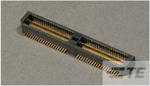
TE 产品编号1658013-2 MSB0.80PL5ASY080FL,-,10,-TY
