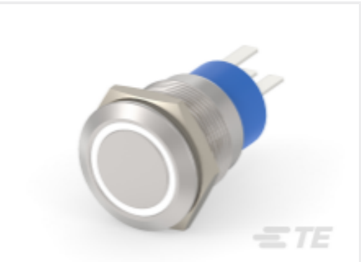
TE 产品编号2213767-3 AV19 SPM 3A MOVE RING LED WHITE 24V
