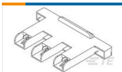
TE 产品编号521823-1 PL 187 HOUSING REC NYLON VO
