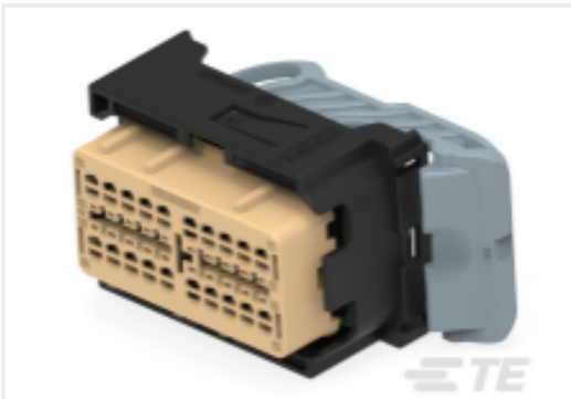
TE 产品编号2322231-1 40POS,HYBRID,REC HSG ASSY,SLD, COD A
