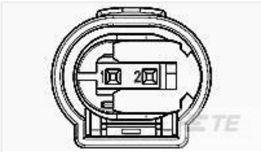
TE 产品编号1-967644-1 2POS MQS REC SEALED COD A
