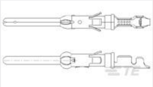
TE 产品编号163086-1 062 PIN ASS. TYP3+
