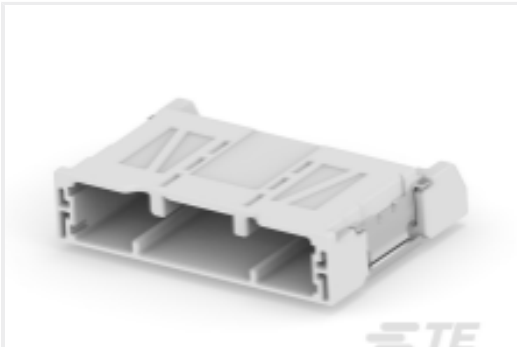
TE 产品编号1939082-9 0.5/1.5 HYBRID 16POS SMT CAP ASSY
