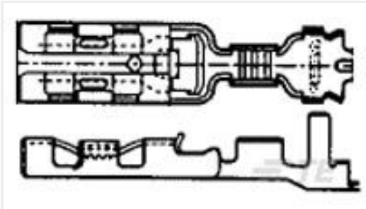
TE 产品编号353249-2 110 PL EX REC. 26-22AWG PTPHBZ
