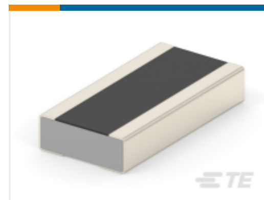
TE 产品编号2176540-2 RLW73 B2 1% R012 600ppm 1k RL
