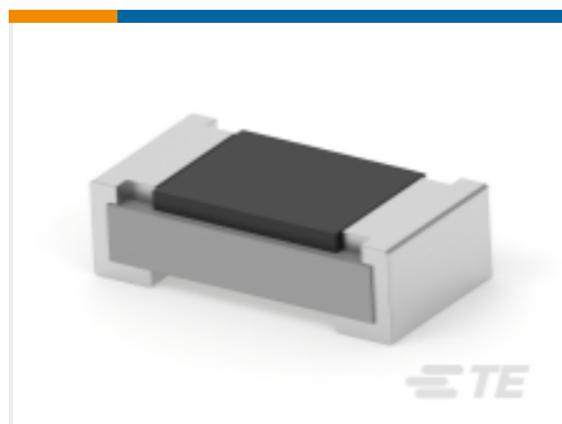
TE 产品编号2176237-6 CPF A 0603 27R 0.1% 25PPM 5K RL
