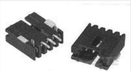
TE 产品编号2306286-5 5P DUOPLUG MARK II SIDE LOCKING, FUL
