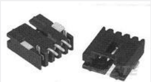
TE 产品编号2306286-4 4P DUOPLUG MARK II SIDE LOCKING, FUL
