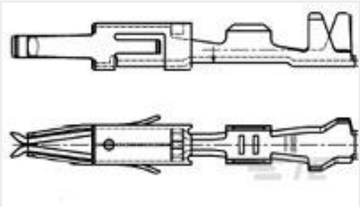
TE 产品编号962943-2 MT2 REC 1.6 Contact SRC Sn
