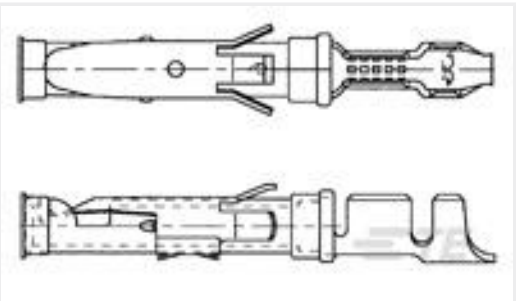
TE 产品编号163087-9 062 SOC.ASS. TYP3+
