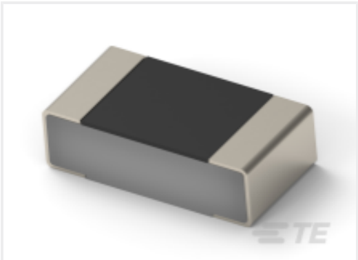
TE 产品编号1-2176467-8 TLRP 1206 1.0W R025 1% 75PPM 5K RL
