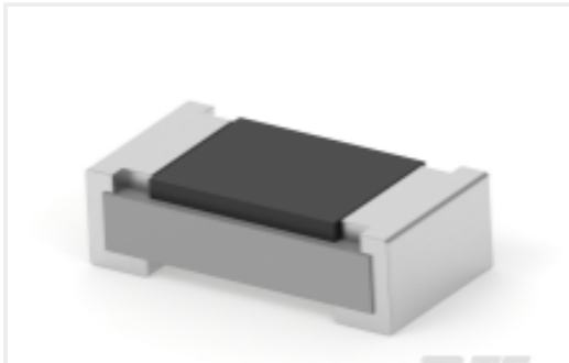
TE 产品编号5-2176237-8 CPF A 0603 75K 0.1% 25PPM 5K RL
