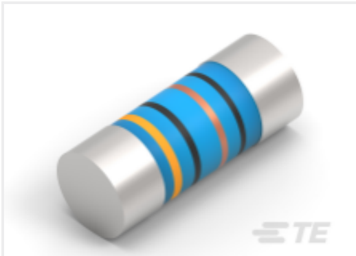
TE 产品编号3-2176315-8 MELF SMA_A 100R 1% 50PPM 0204 0.4 W
