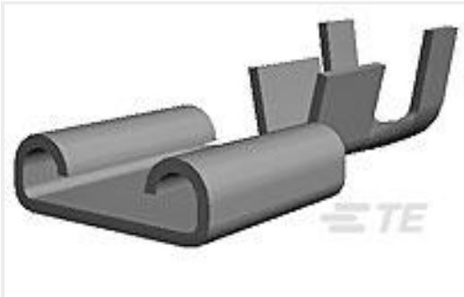
TE 产品编号170183-1 250 FASTON,REC.,22-18 AWG,BR
